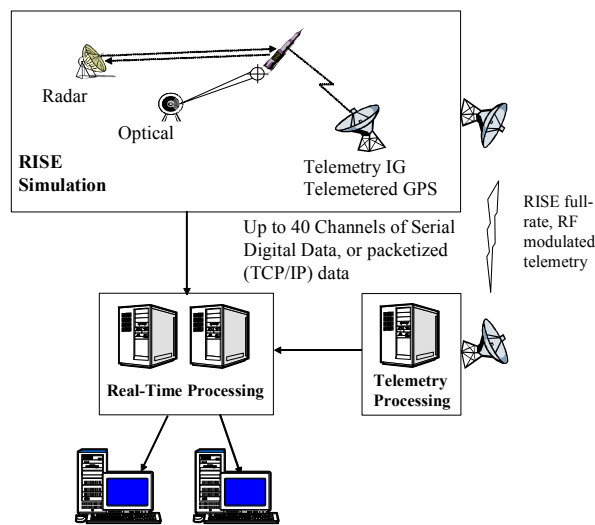
Figure 2 – RISE Concept within Range
