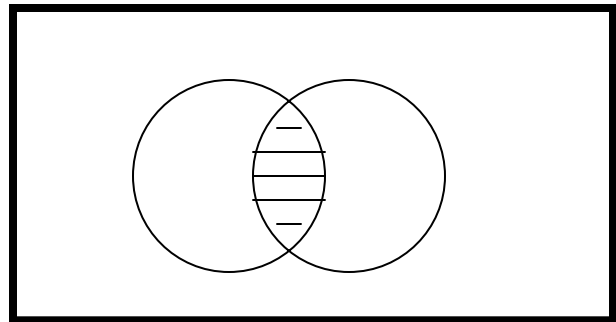
Figure 3. An Intersection of Two Sets
